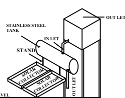
SOLAR HEATING WATER SYSTEM
