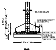
COLUMN FOOTING DETAILS
