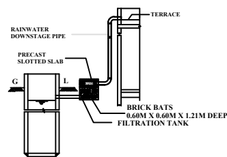
RAIN WATER HARVESTING SYSTEM
