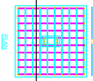
COLUMN FOUNDATION DETAILS
