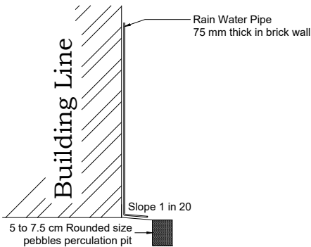
RAINWATER HARVESTING
