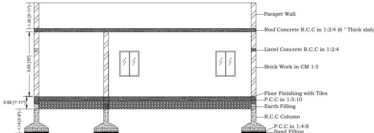
SECTION X-X
