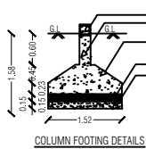
COLUMN FOOTING DETAILS
