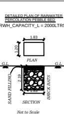
DETAILS OF PLAN OF RAINWATER DISPOSAL SYSTEM
