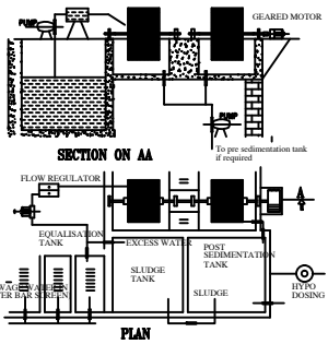
SEWAGE TREATMENT PLANT DETAILS
