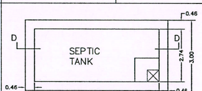
PLAN OF SEPTIC TANK SCALE 1"=2'0"
