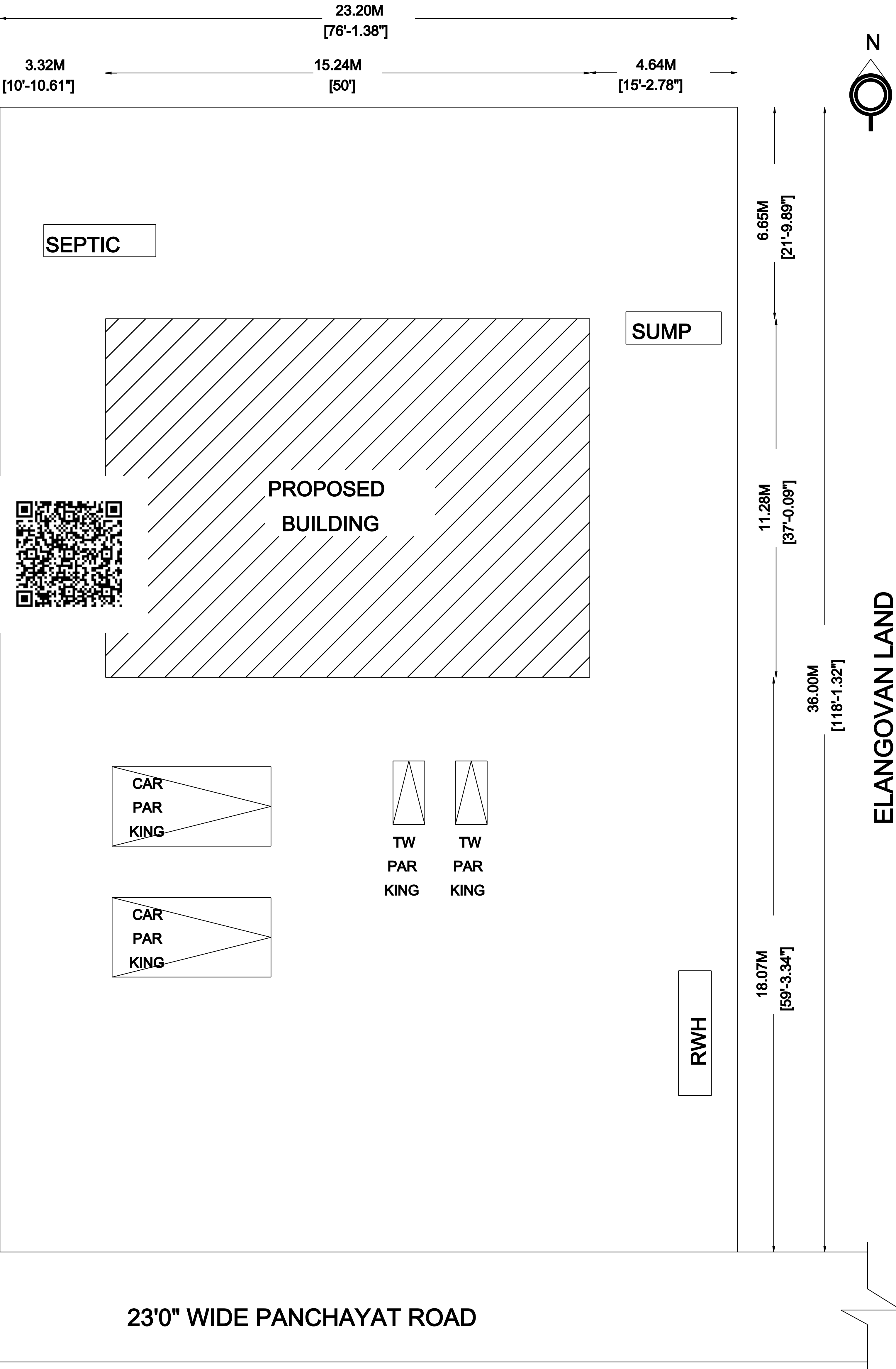
SITE PLAN NOT TO SCALE
