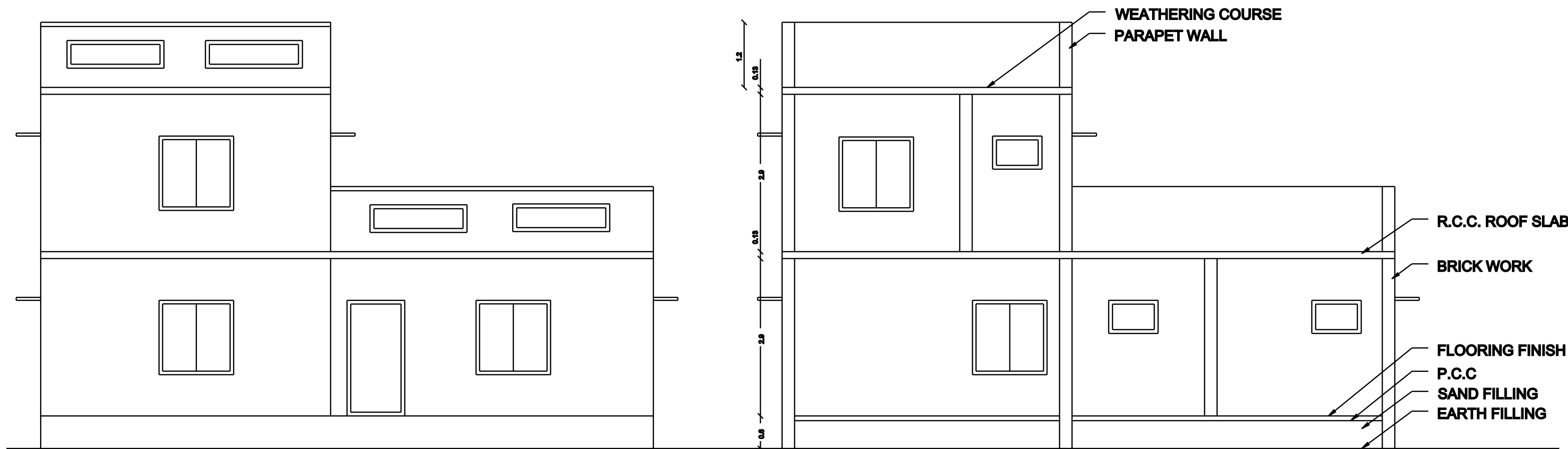
FRONT ELEVATION
