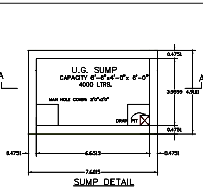
SUMP DETAIL
