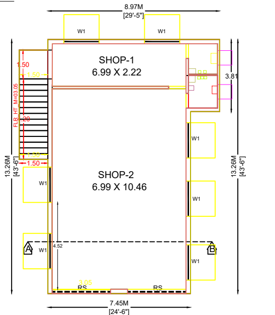
PROPOSED GROUND FLOOR PLAN(SHOP)
