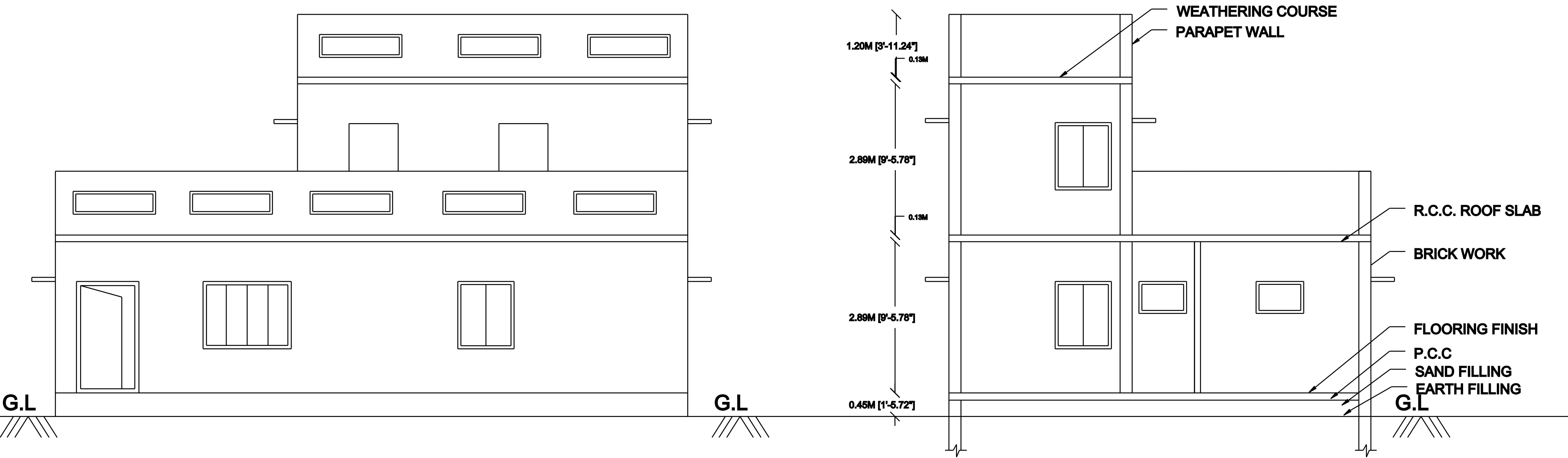
FRONT ELEVATION
