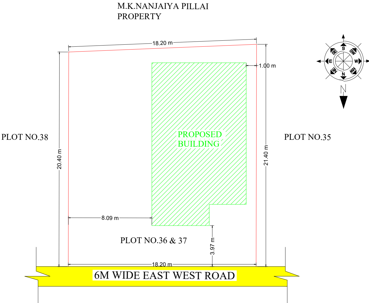
SITE PLAN
