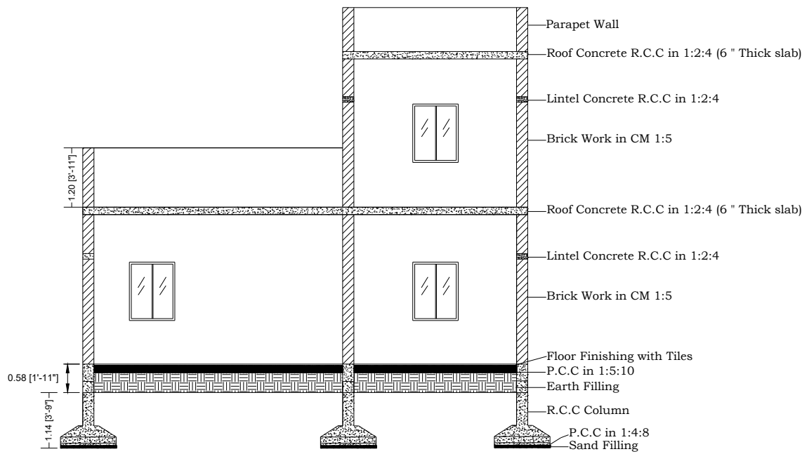
SECTION X-X
