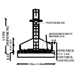
TYP.DET. COLUMN FOOTING
