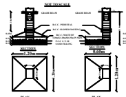
COLUMNS FOOTING DETAILS
