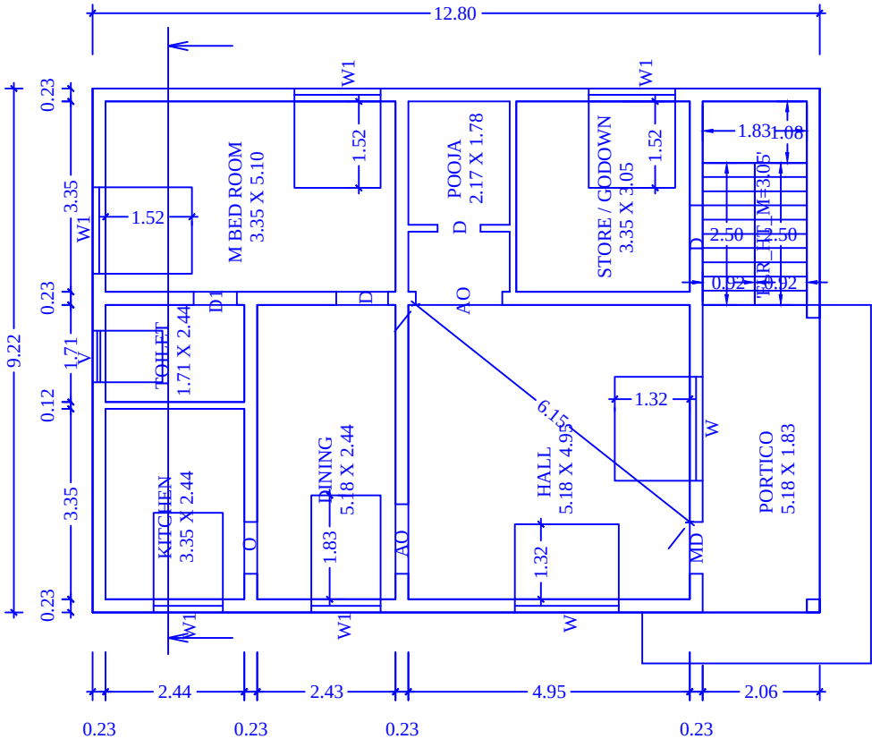
PLAN FOR GROUND FLOOR
