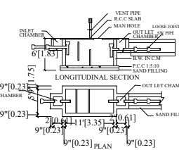
SEPTIC TANK
