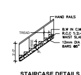
STAIRCASE DETAILS
