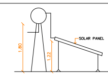
SIDE ELEVATION (NOT TO SCALE)
