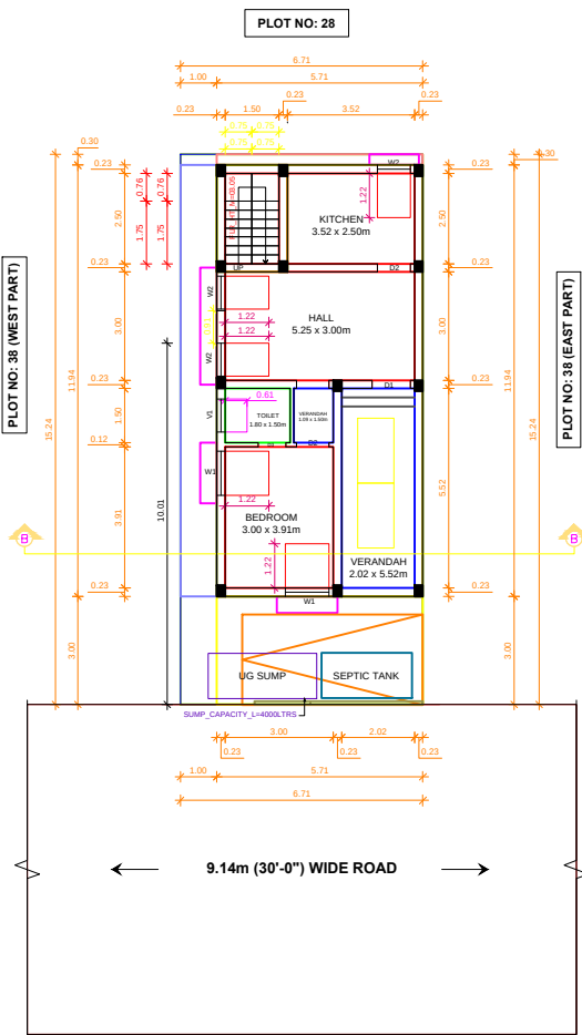
SITE CUM GROUND FLOOR PLAN
