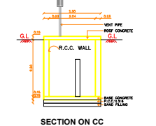
SECTION ON CC
