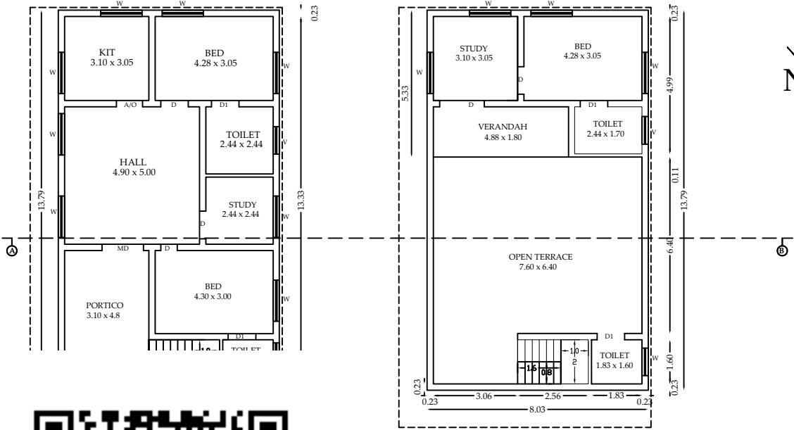
FIRST FLOOR
