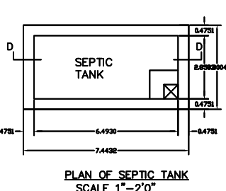
PLAN OF SEPTIC TANK SCALE 1"=2'0"
