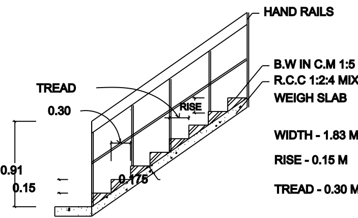
STAIR CASE DETAILS: SCALE 1 : 50
