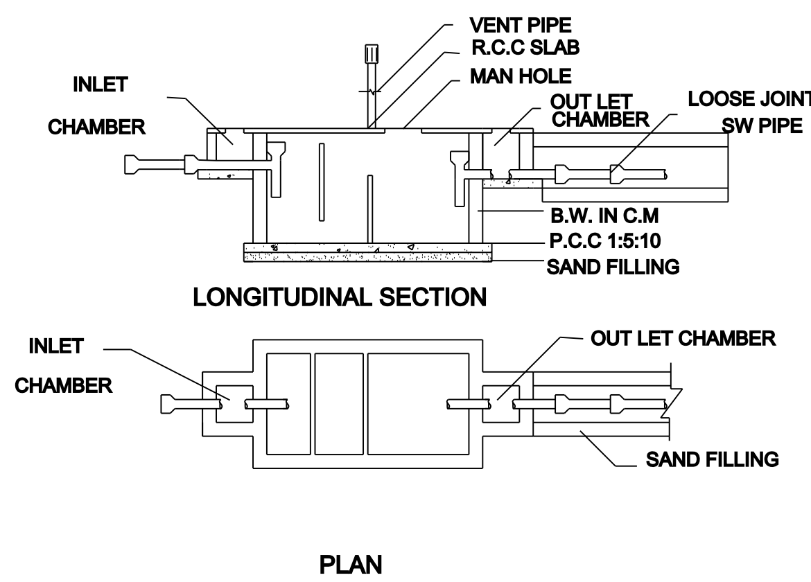
SEPTIC TANK:
