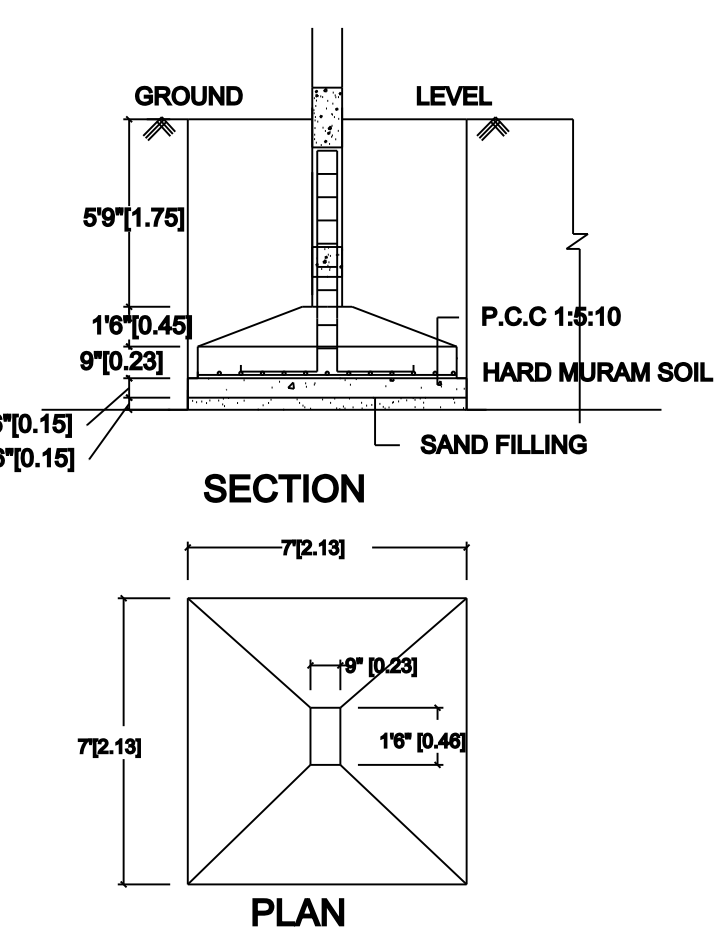
FOUNDATION DETAILS
