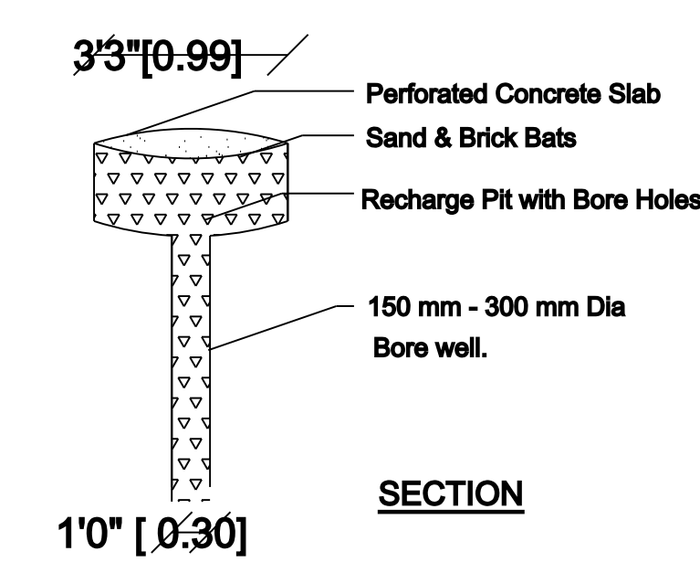
CONSERVATION OF RAIN WATER
