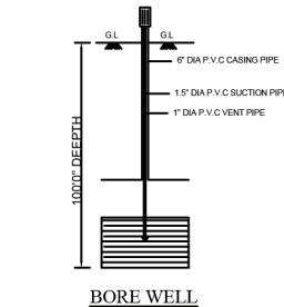
BORE WELL
