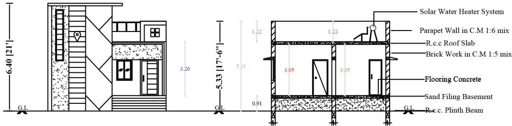
FRONT ELEVATION
