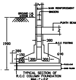
TYPICAL SECTION OF R.C.C COLUMN FOUNDATION
