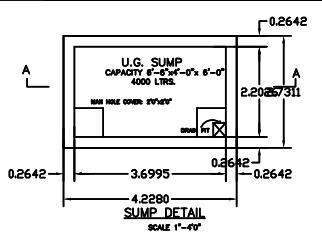
SUMP DETAIL
