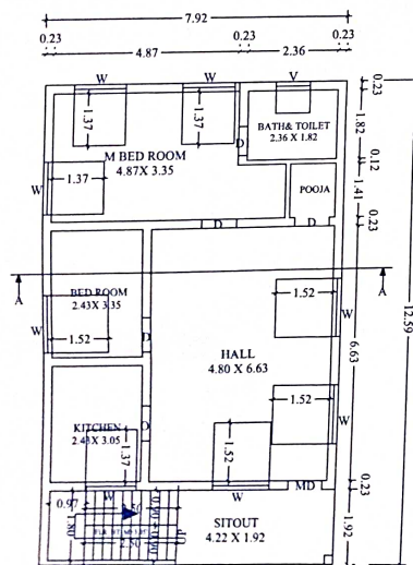
PLAN FOR GROUND FLOOR
