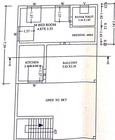
PLAN FOR FIRST FLOOR
