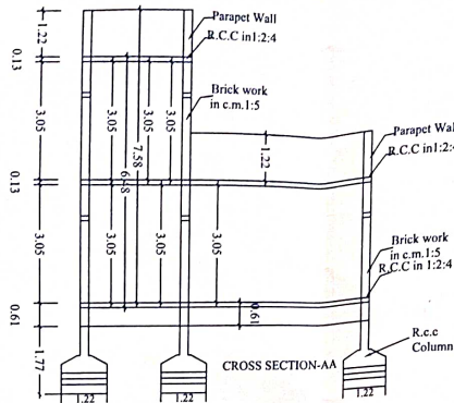
CROSS SECTION-AA
