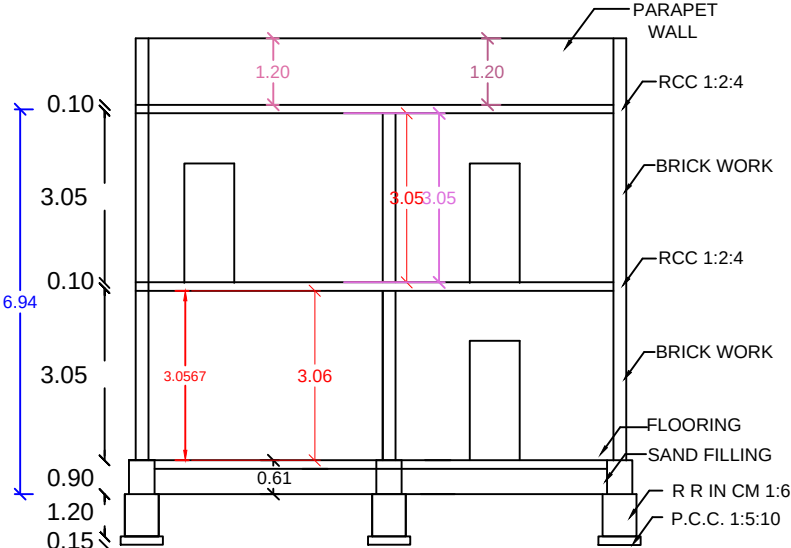
SECTION AB
