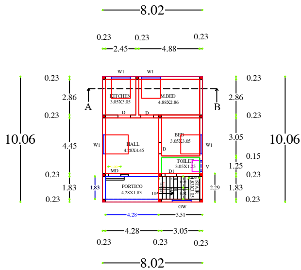
PRO.GROUND FLOOR PLAN NORTH FACING
