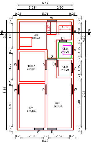
EXISTING & PROPOSED GROUND FLOOR PLAN
