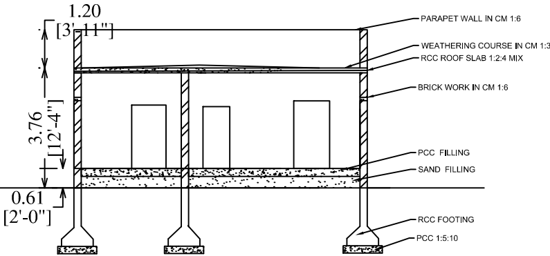
SEC ON -XY
