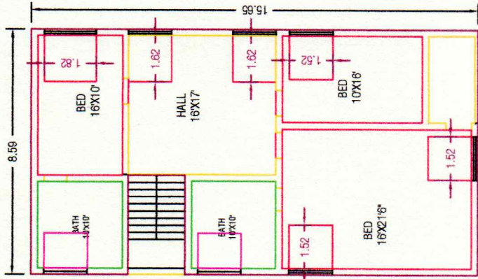
FLOOR-FIRST PROPOSED FIRST FLOOR PLAN
