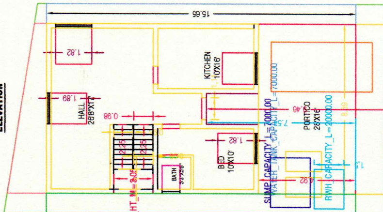
FLOOR-GROUND PROPOSED GROUND FLOOR PLAN
