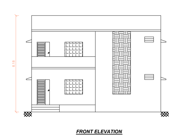
FRONT ELEVATION
