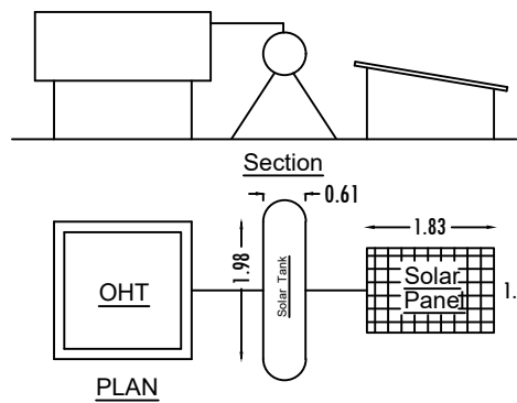
Solar System
