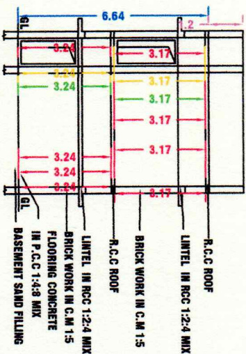
CROSS SECTION ON "A-A"
