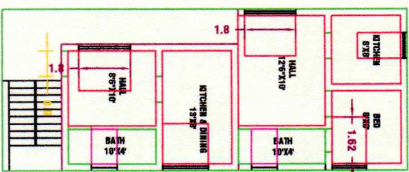
FLOOR-FIRST PROPOSED FIRST FLOOR PLAN
