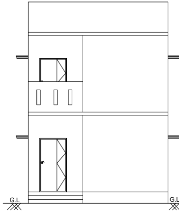
ELEVATION ON A-A
