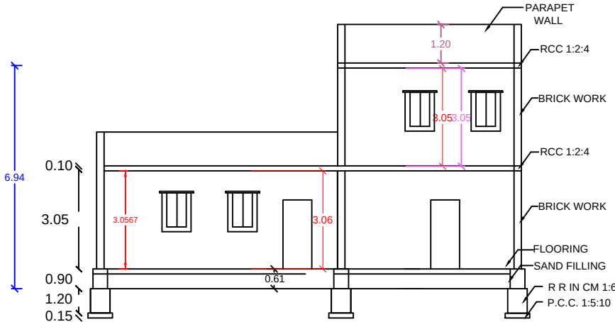
SECTION AB
