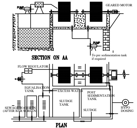
SEWAGE TREATMENT PLANT DETAILS
