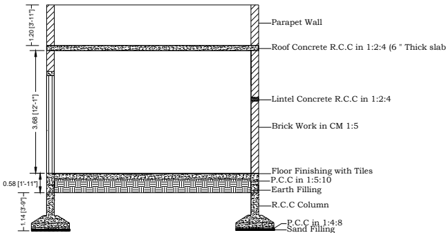
SECTION X-X
