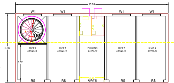
EXISTING GROUND FLOOR
