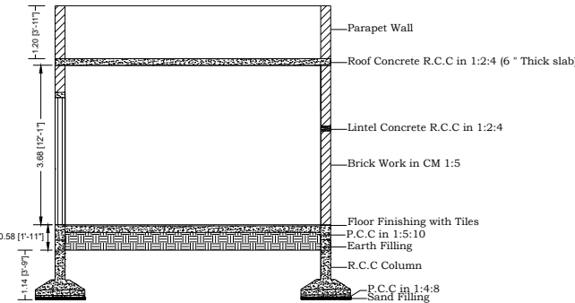
SECTION X-X
