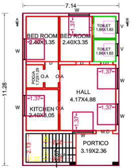
GROUND FLOOR PLAN SCALE 1:100 FLR_HT_M=3.05
