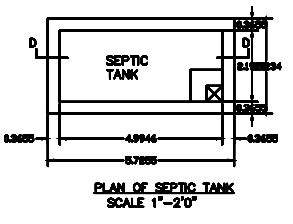
PLAN OF SEPTIC TANK SCALE 1"=2'-0"
