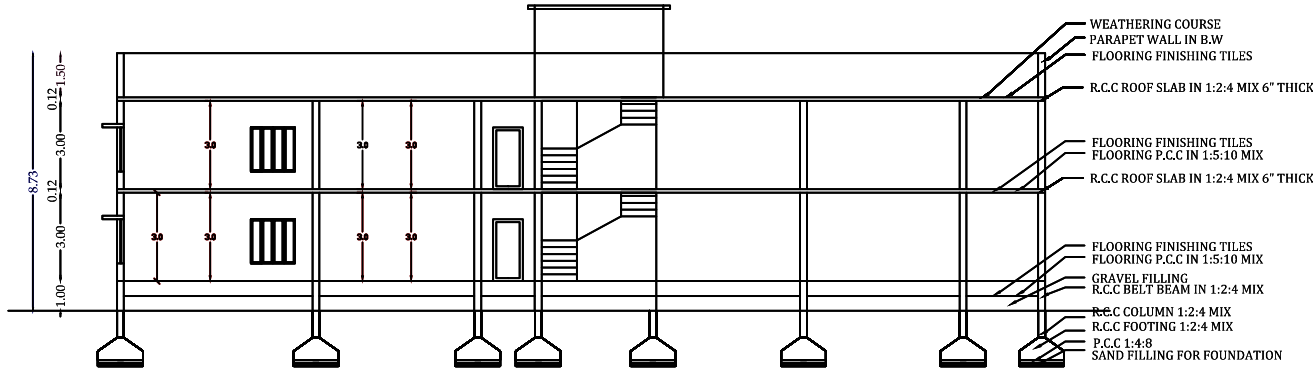
SECTION A TO B
