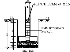
COLUMN & FOOTING DETAIL
