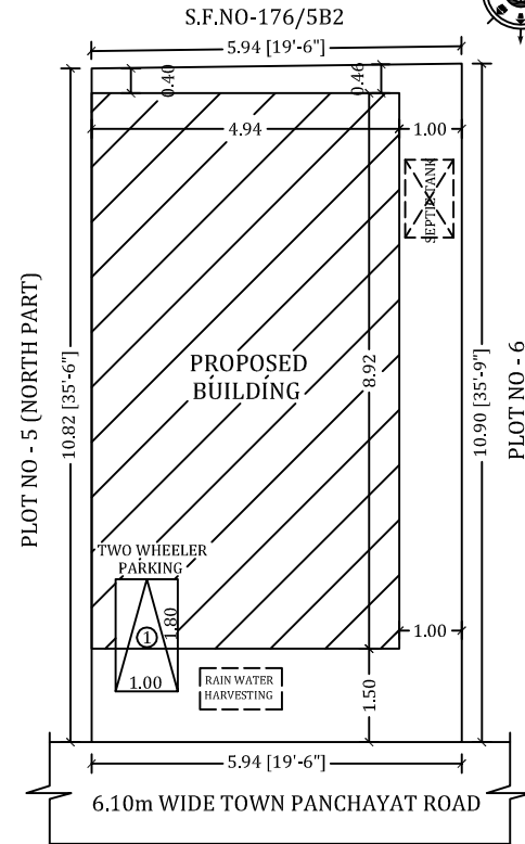
SITE PLAN
