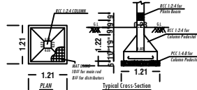
FOOTING DETAILS
