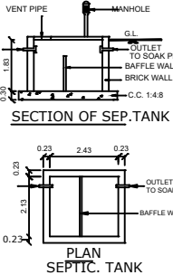
SEPTIC TANK:-
