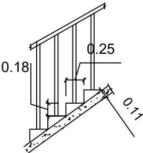
STAIRCASE DETAILS:-
