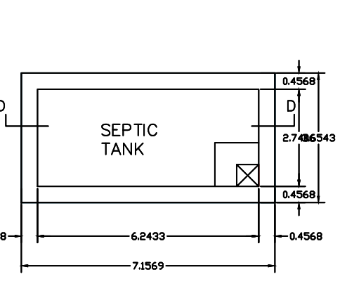
PLAN OF SEPTIC TANK SCALE 1"=2'0"
