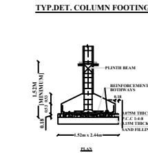
TYP.DET. COLUMN FOOTING
