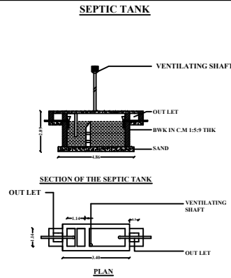
SEPTIC TANK
