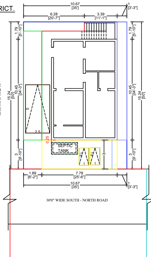
Details of Waste Water Recycling Tank - Kitchen, Bath Waste Water Reuse Method
