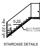
STAIRCASE DETAILS
