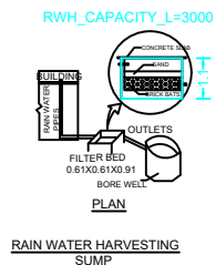
RAIN WATER HARVESTING SUMP
