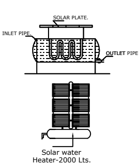
Solar water Heater-2000 Lts.
