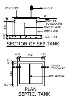
PLAN SEPTIC. TANK
