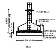
TYP.DET. COLUMN FOOTING
