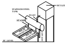
SOLAR HEATING WATER SYSTEM
