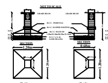
COLUMN FOOTING DETAILS
