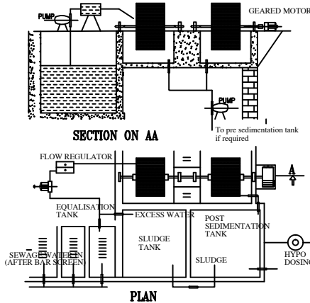
SEWAGE TREATMENT PLANT DETAILS
