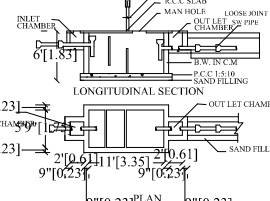
SEPTIC TANK:
