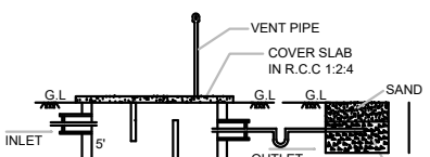
SECTION-AB
