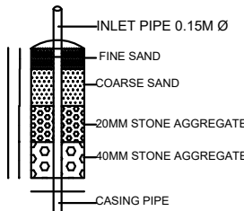
DETAILS OF RAIN WATER
