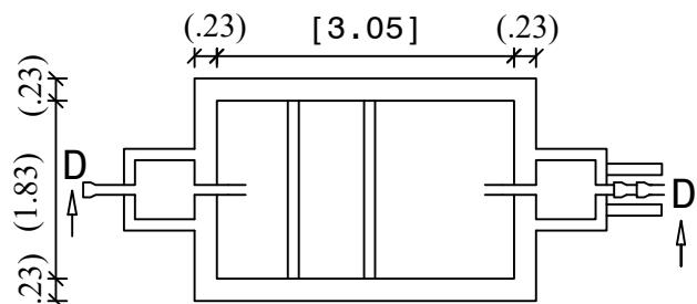
SEPTIC TANK PLAN
