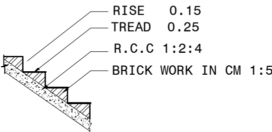
STAIRCASE DETAILS
