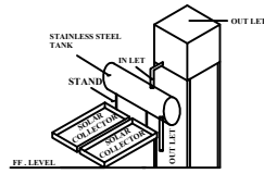
SOLAR HEATING WATER SYSTEM
