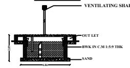
SECTION OF THE SEPTIC TANK
