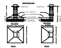
COLUMN FOOTING DETAILS
