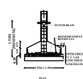
TYP.BET. COLUMN FOOTING
