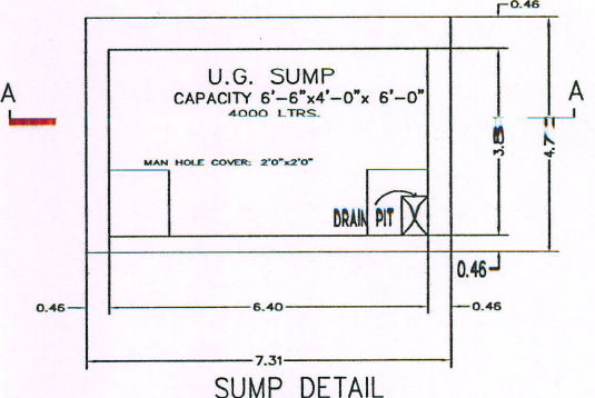
SUMP DETAIL SCALE 1"-4'0"
