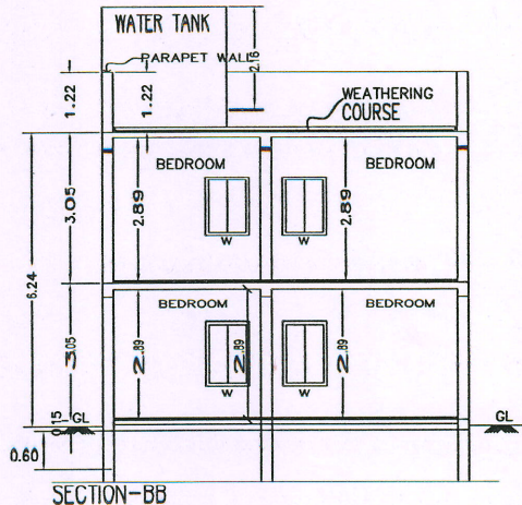
SECTION-BB
