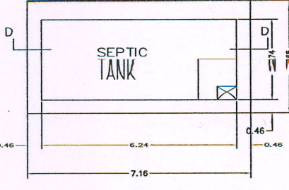
PLAN OF SEPTIC TANK SCALE 1"-2'0"
