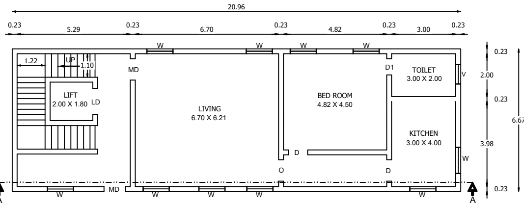
GROUND FLOOR
