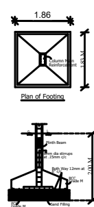
FOUNDATION DETAILS
