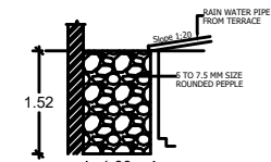
RAINWATER HARVESTING TRENCH
