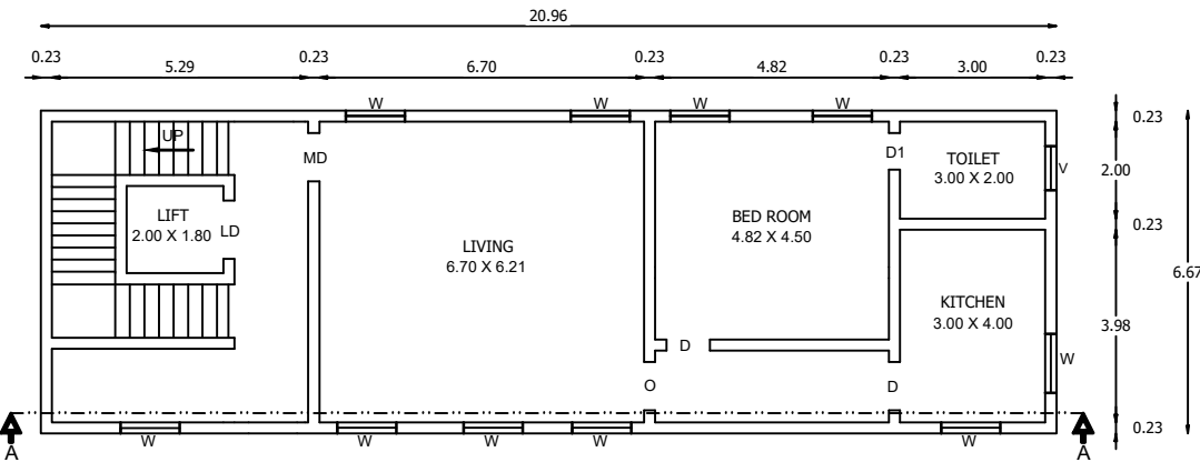
TYPICAL 1ST.2ND.FLOOR
